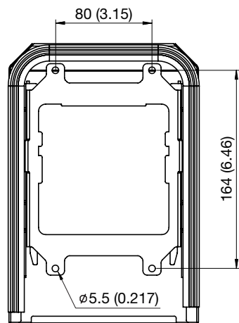
Mounting cut-out mm (in)
